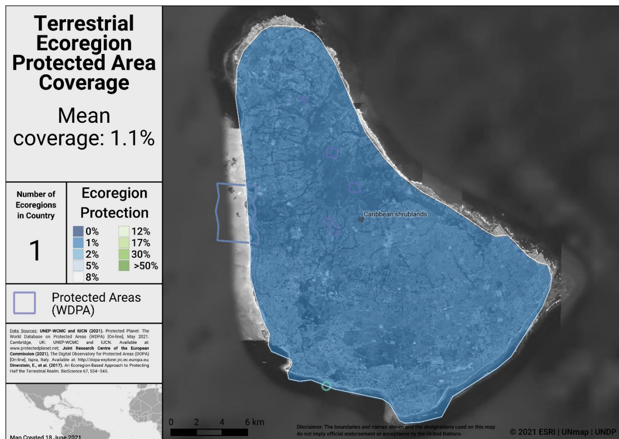
Terrestrial ecoregions in Barbados
