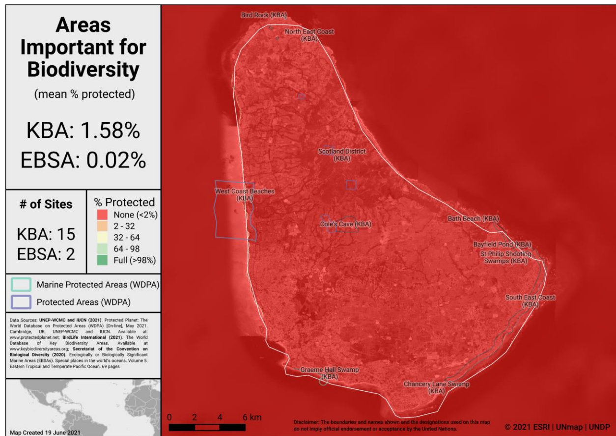
Areas Important for Biodiversity in Barbados
