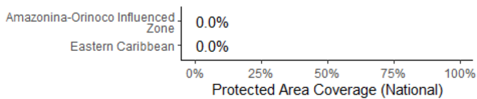
Ecologically or Biologically Significant Marine Areas (EBSAs) in Barbados
